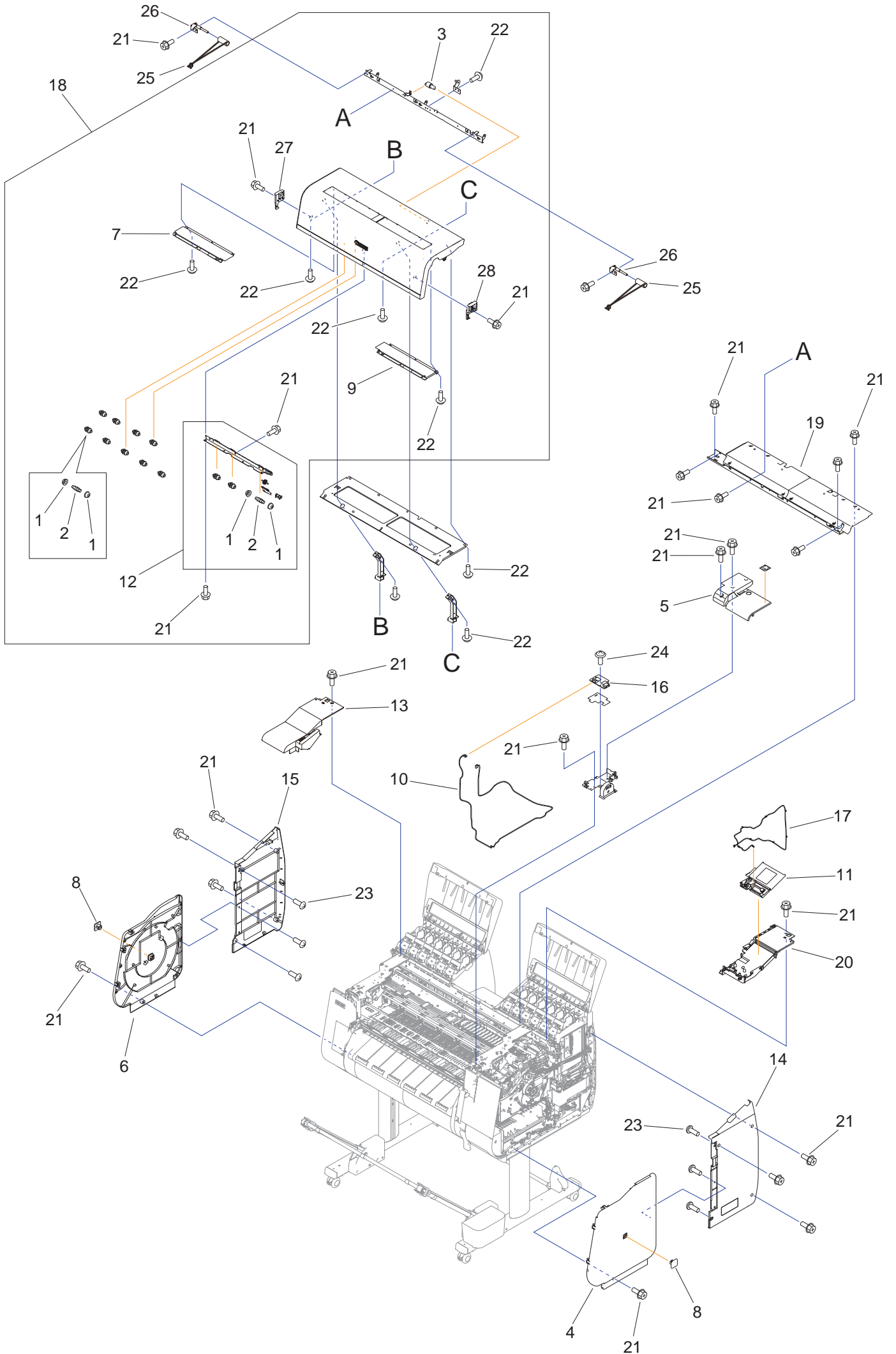
Figure 02 TOP COVERS & SIDE COVERS
