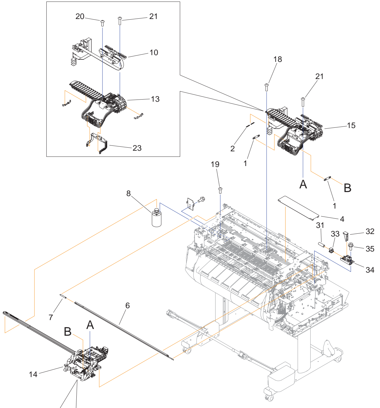
Figure 06 CARRIAGE, TUBE UNIT & FILM STRIP
