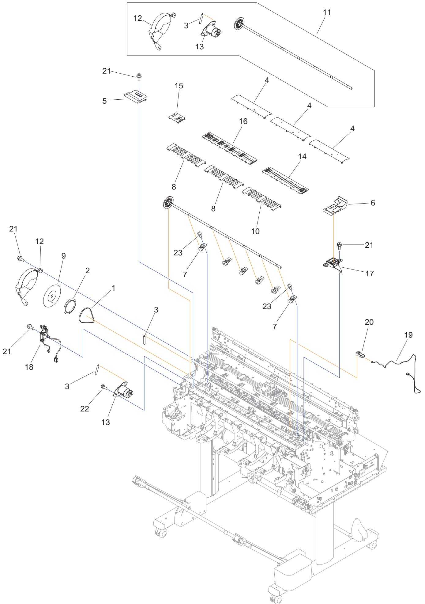
Figure 10 PLATEN & FEED ROLLER
